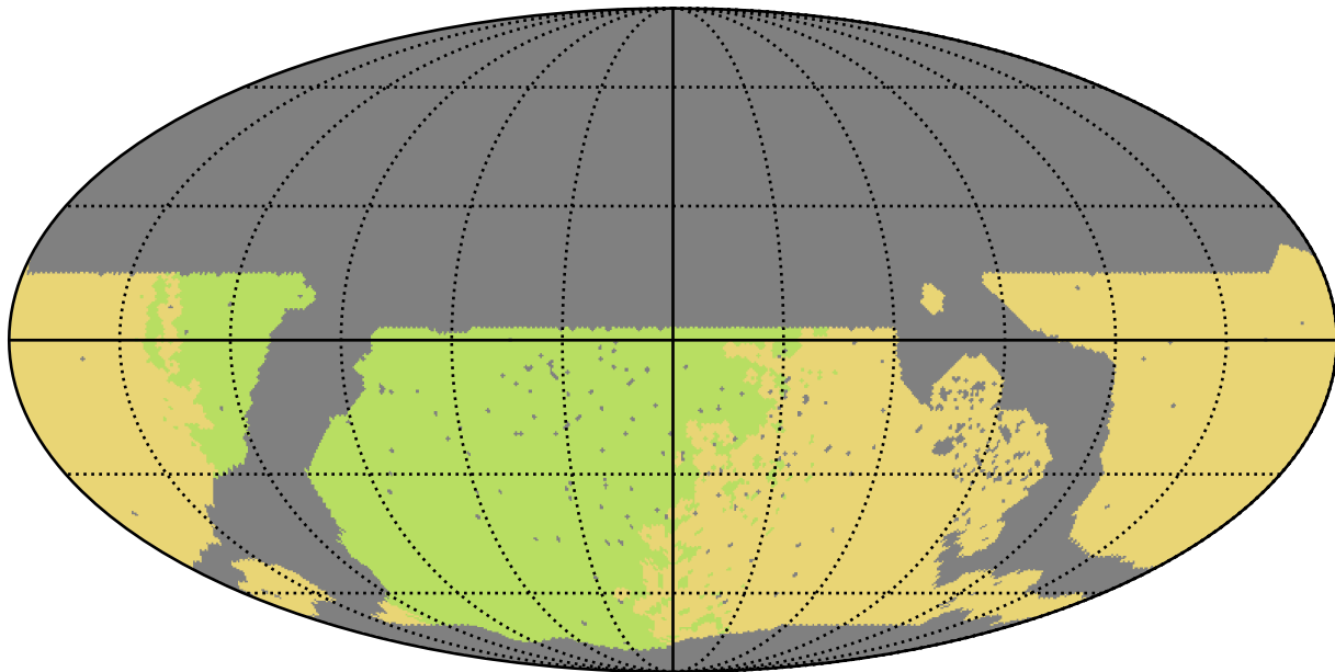
noroll_v3.4_10yrs WFD all bands: NSeasons
