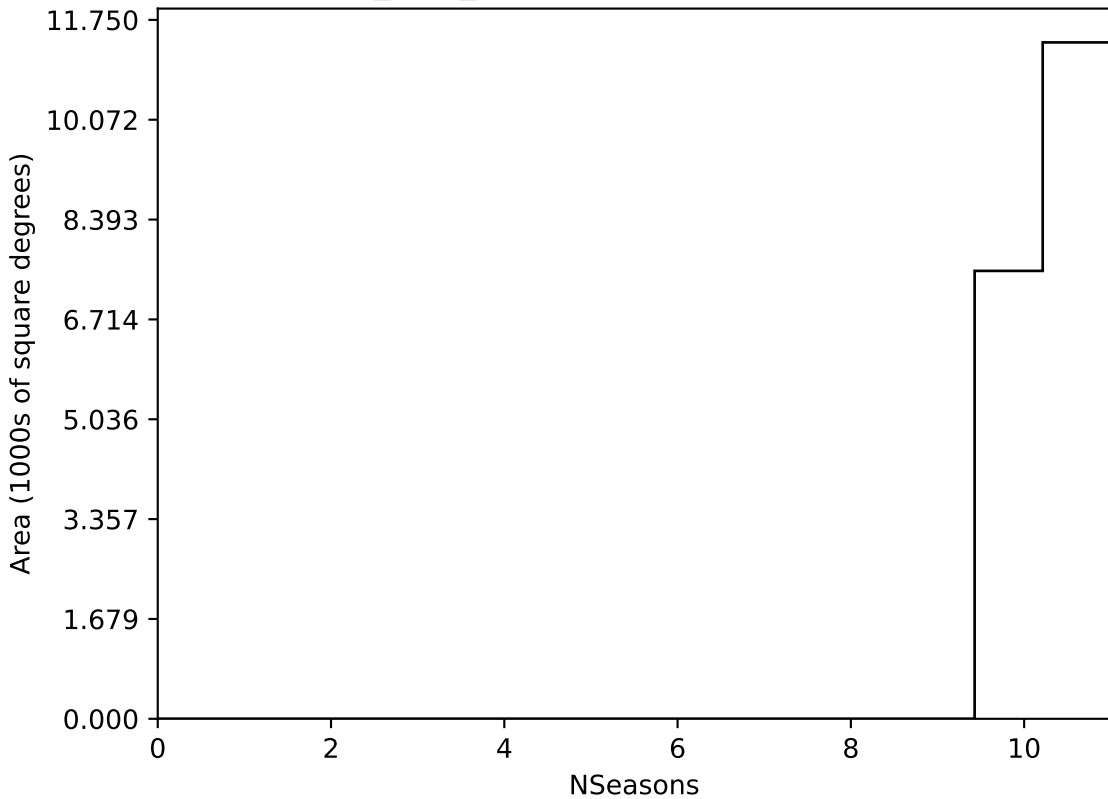
noroll_v3.4_10yrs WFD all bands: NSeasons
