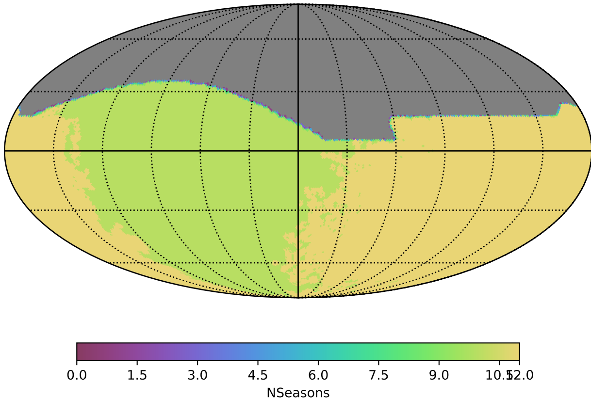
noroll_v3.4_10yrs All sky all bands: NSeasons
