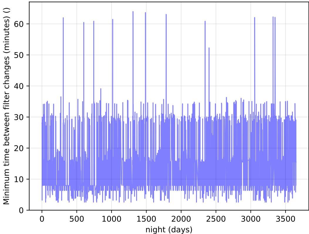
noroll_v3.4_10yrs Per Night: Minimum time between filter changes (minutes)
