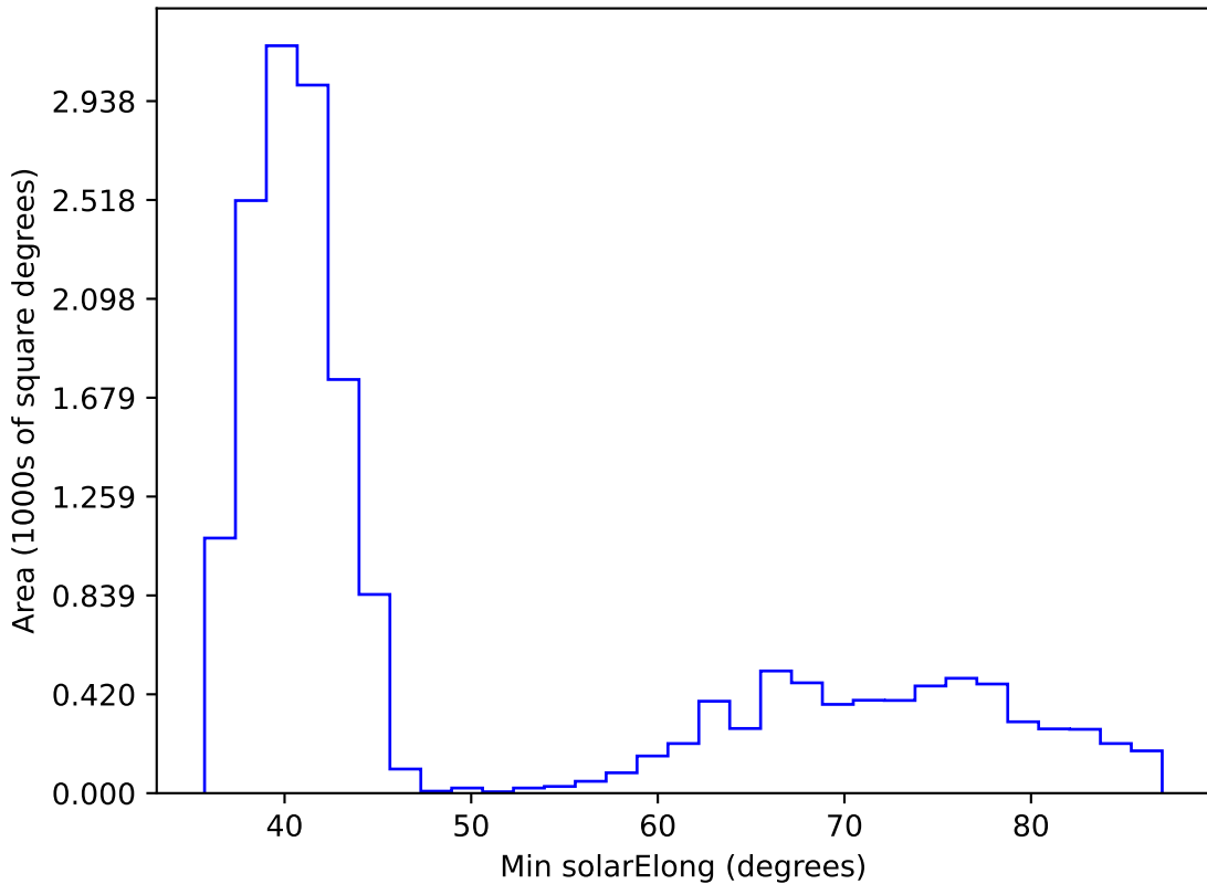
noroll_v3.4_10yrs WFD z band: Min solarElong
