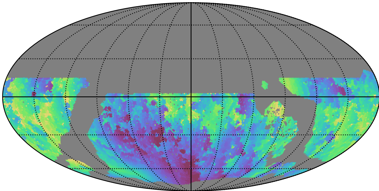
noroll_v3.4_10yrs WFD u band: Min solarElong
