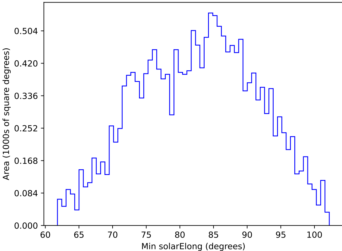
noroll_v3.4_10yrs WFD u band: Min solarElong
