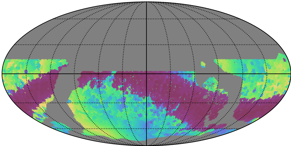
noroll_v3.4_10yrs WFD r band: Min solarElong
