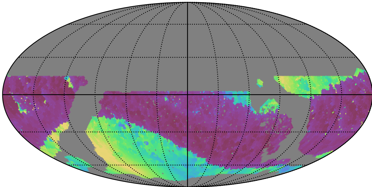
noroll_v3.4_10yrs WFD i band: Min solarElong
