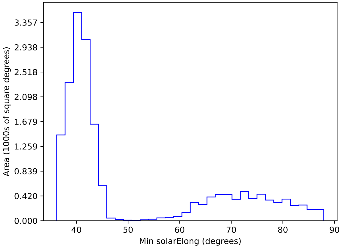
noroll_v3.4_10yrs WFD i band: Min solarElong
