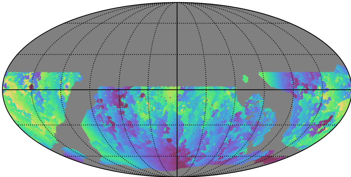
noroll_v3.4_10yrs WFD g band: Min solarElong
