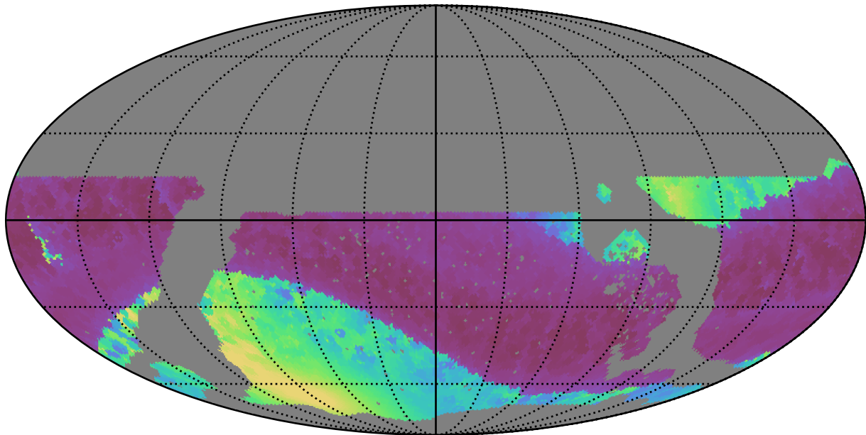
noroll_v3.4_10yrs WFD all bands: Min solarElong
