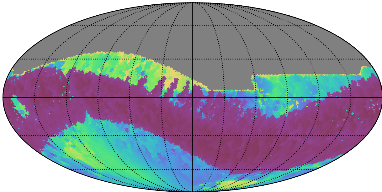
noroll_v3.4_10yrs All sky z band: Min solarElong
