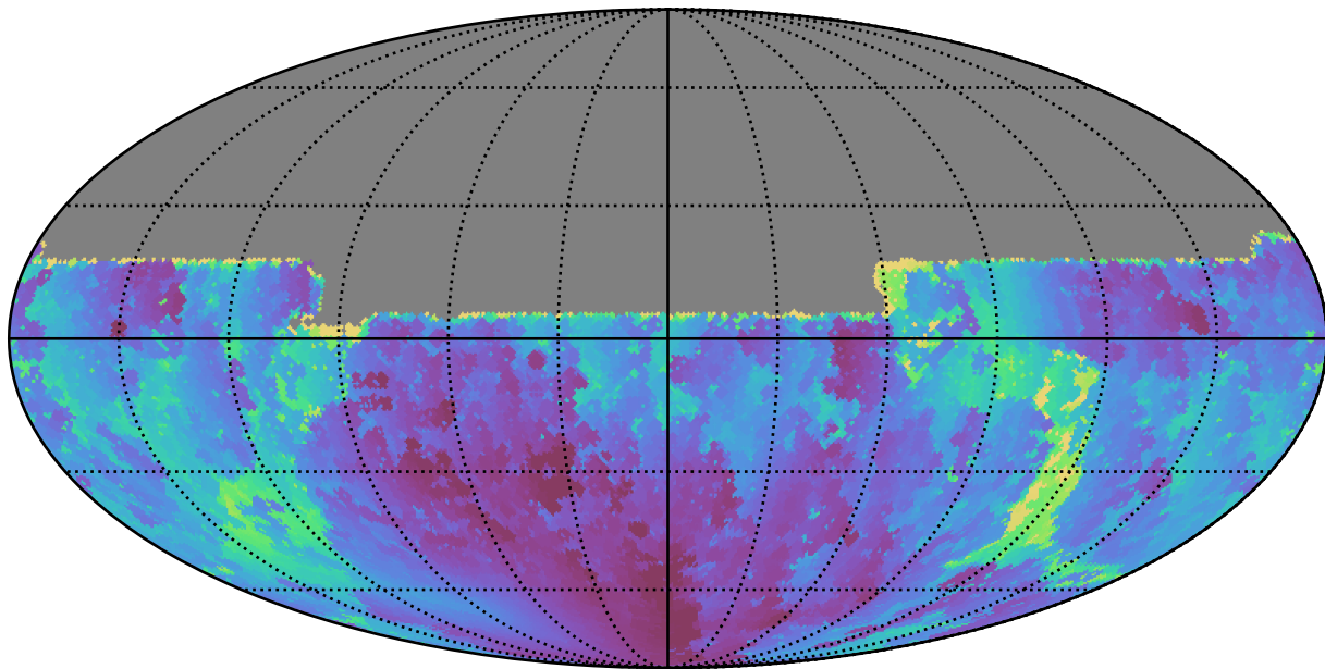
noroll_v3.4_10yrs All sky u band: Min solarElong
