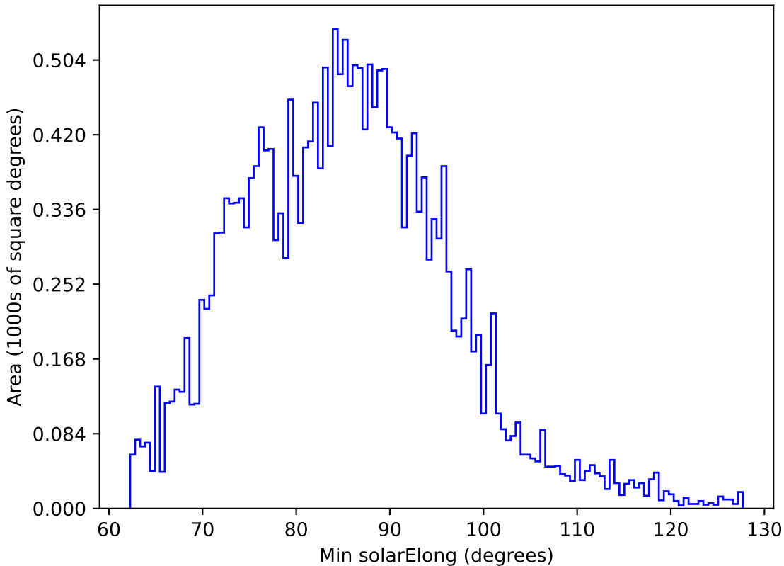
noroll_v3.4_10yrs All sky u band: Min solarElong
