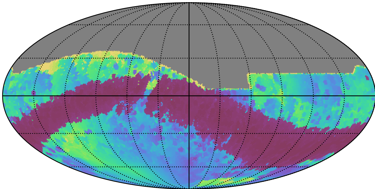
noroll_v3.4_10yrs All sky r band: Min solarElong
