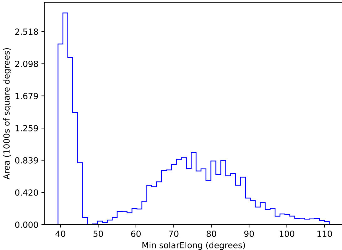
noroll_v3.4_10yrs All sky r band: Min solarElong
