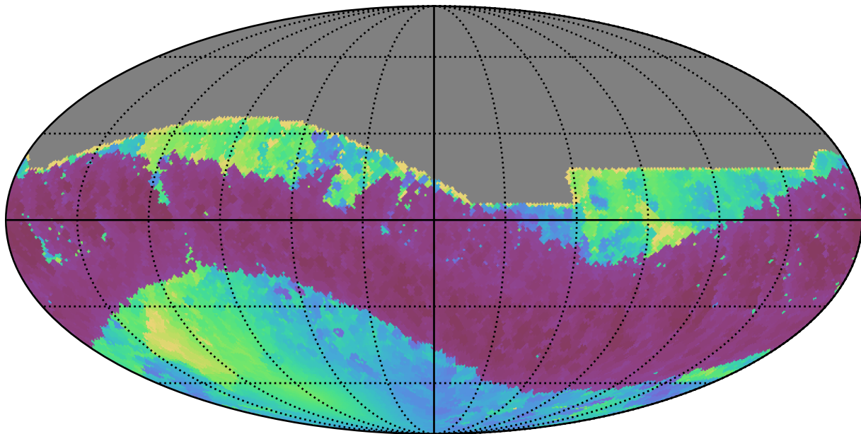
noroll_v3.4_10yrs All sky i band: Min solarElong
