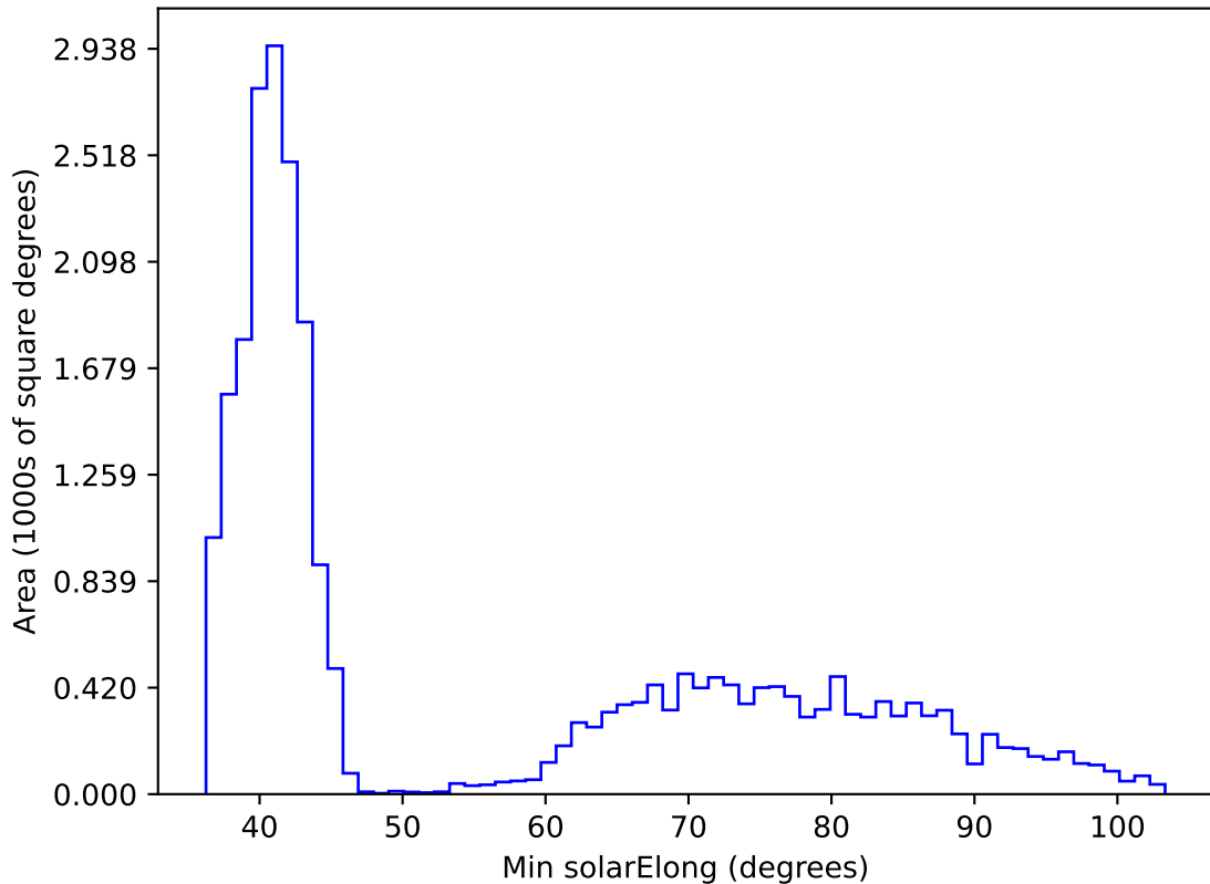
noroll_v3.4_10yrs All sky i band: Min solarElong
