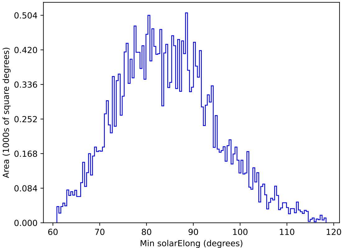
noroll_v3.4_10yrs All sky g band: Min solarElong
