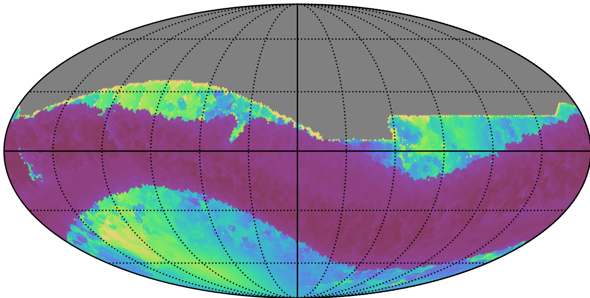
noroll_v3.4_10yrs All sky all bands: Min solarElong
