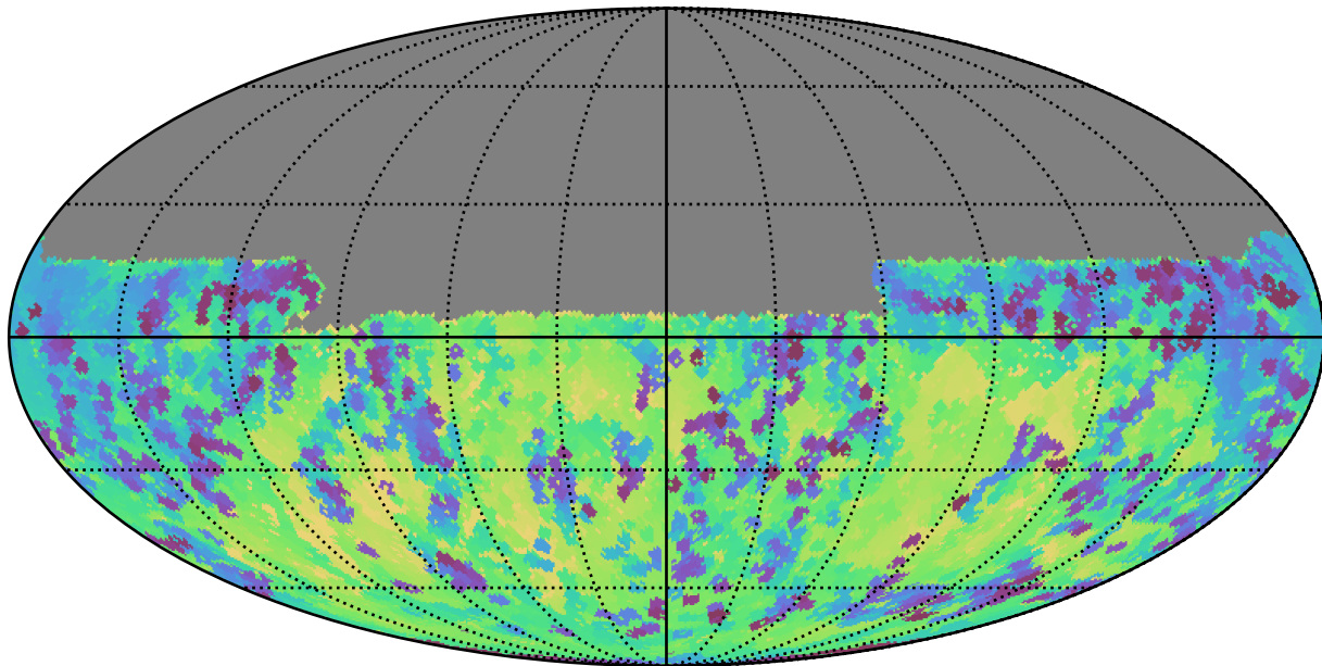
noroll_v3.4_10yrs Yr 1 y band: Min skyBrightness
