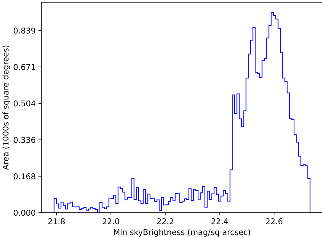
noroll_v3.4_10yrs Yr 1 u band: Min skyBrightness
