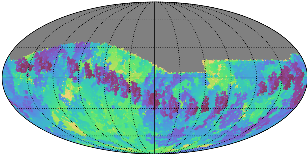
noroll_v3.4_10yrs Yr 1 i band: Min skyBrightness
