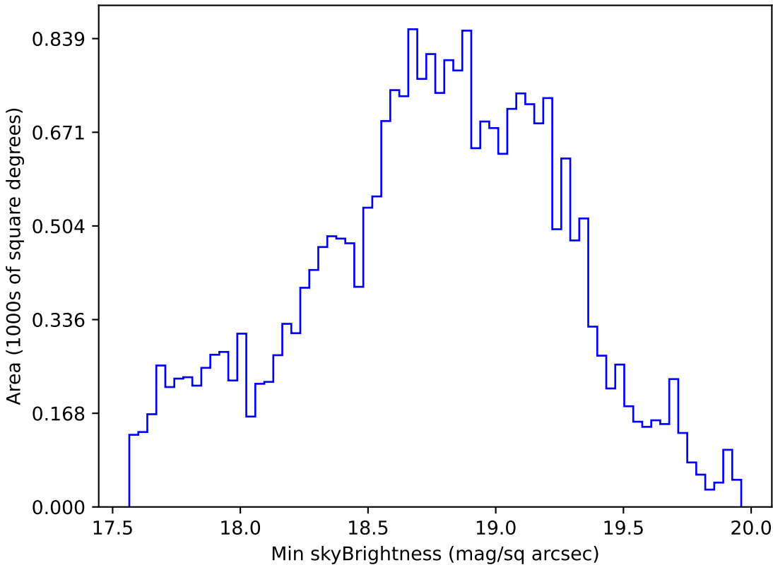
noroll_v3.4_10yrs Yr 1 i band: Min skyBrightness
