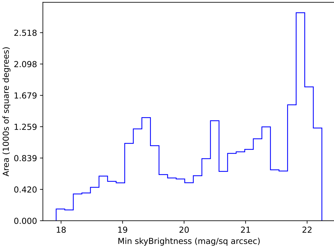
noroll_v3.4_10yrs Yr 1 g band: Min skyBrightness
