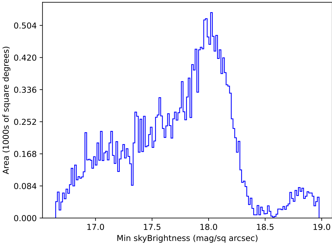
noroll_v3.4_10yrs Yr 1 all bands: Min skyBrightness
