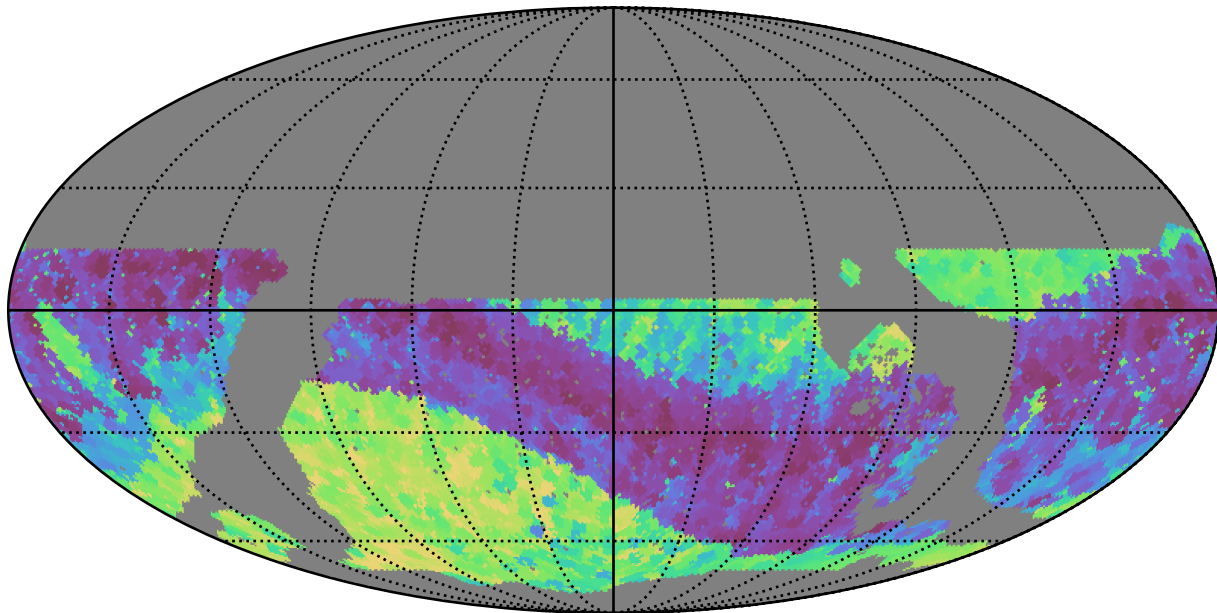
noroll_v3.4_10yrs WFD z band: Min skyBrightness
