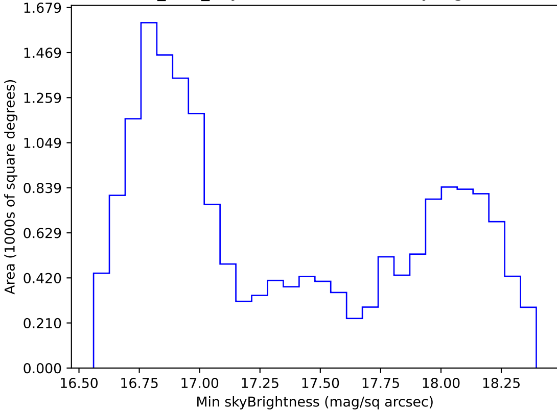
noroll_v3.4_10yrs WFD z band: Min skyBrightness
