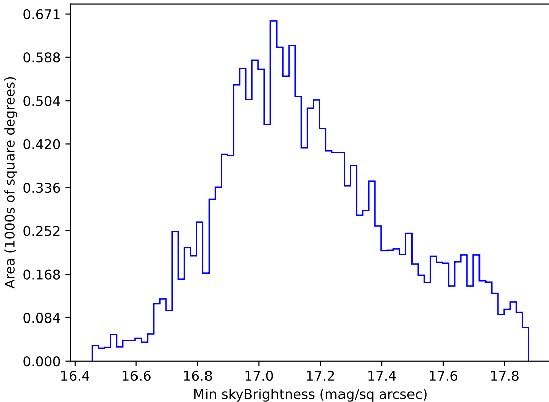
noroll_v3.4_10yrs WFD y band: Min skyBrightness
