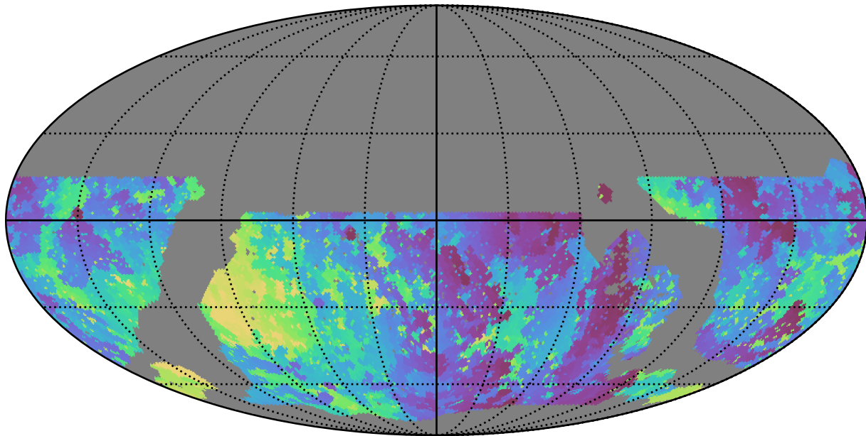
noroll_v3.4_10yrs WFD u band: Min skyBrightness
