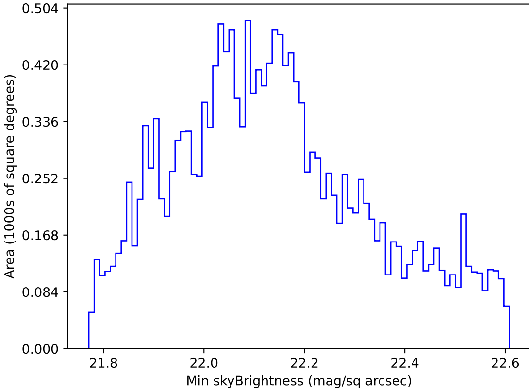
noroll_v3.4_10yrs WFD u band: Min skyBrightness
