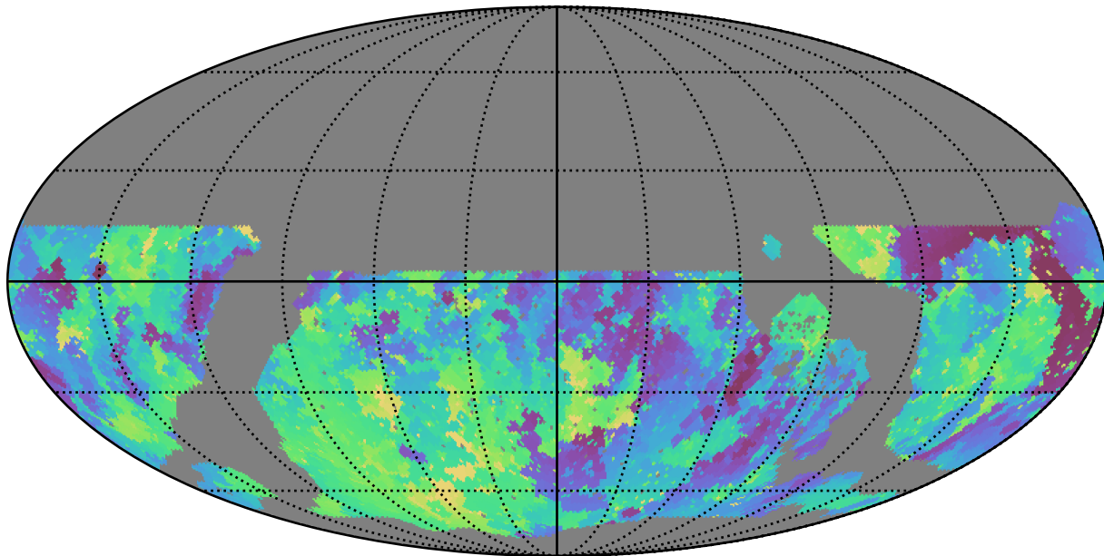
noroll_v3.4_10yrs WFD r band: Min skyBrightness
