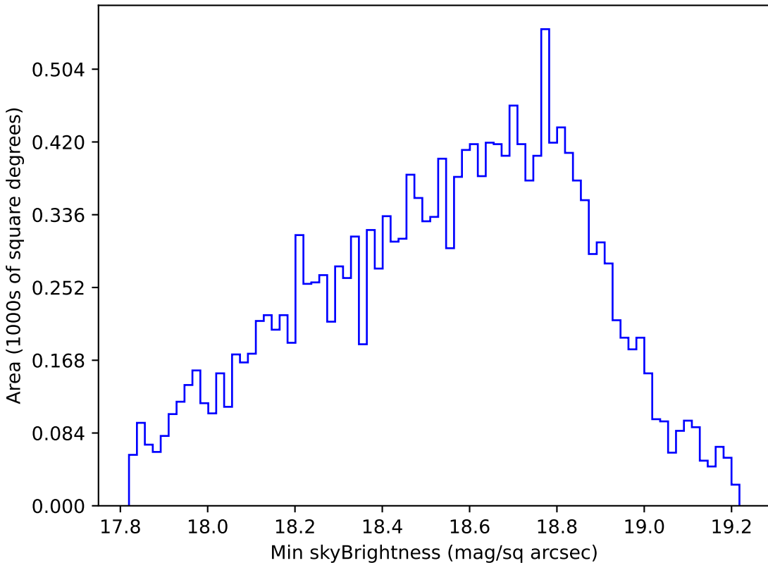
noroll_v3.4_10yrs WFD r band: Min skyBrightness
