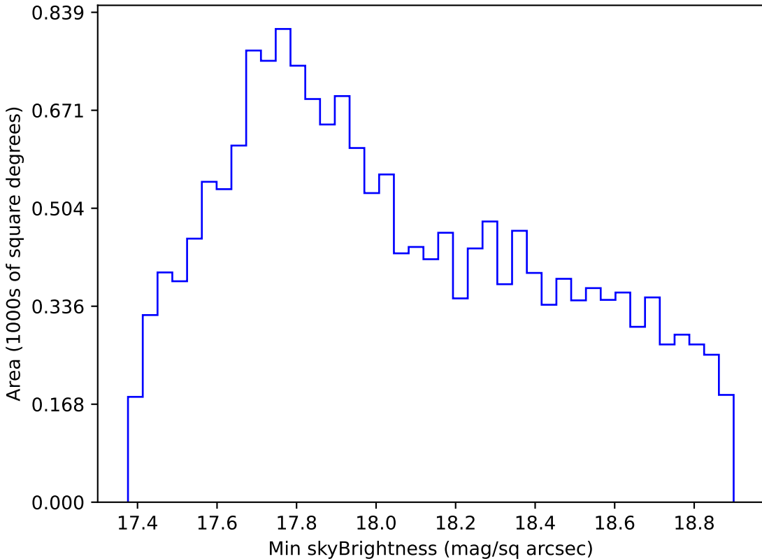
noroll_v3.4_10yrs WFD i band: Min skyBrightness
