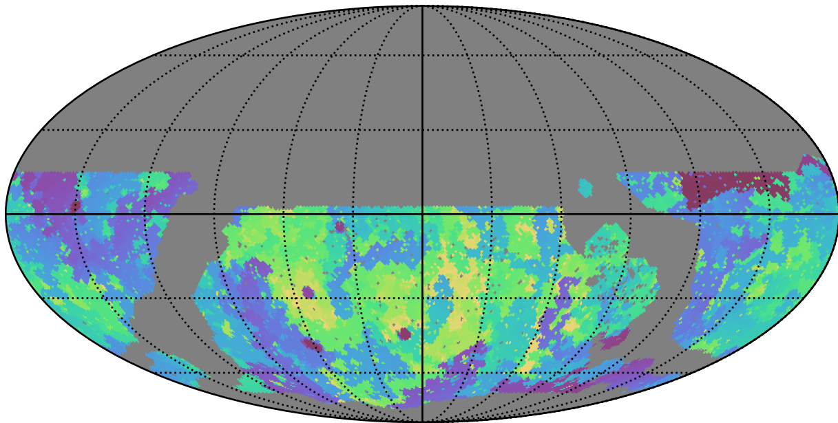
noroll_v3.4_10yrs WFD g band: Min skyBrightness
