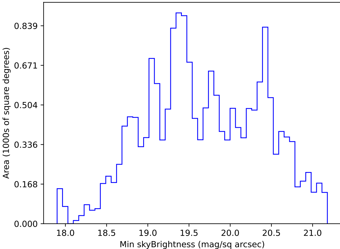
noroll_v3.4_10yrs WFD g band: Min skyBrightness
