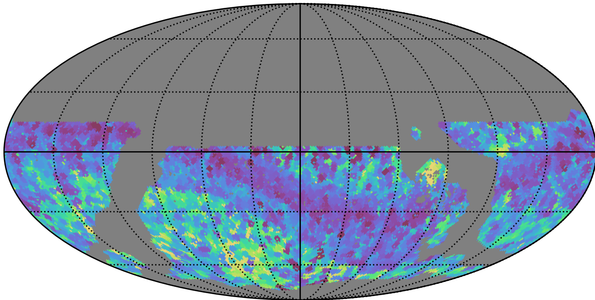
noroll_v3.4_10yrs WFD all bands: Min skyBrightness
