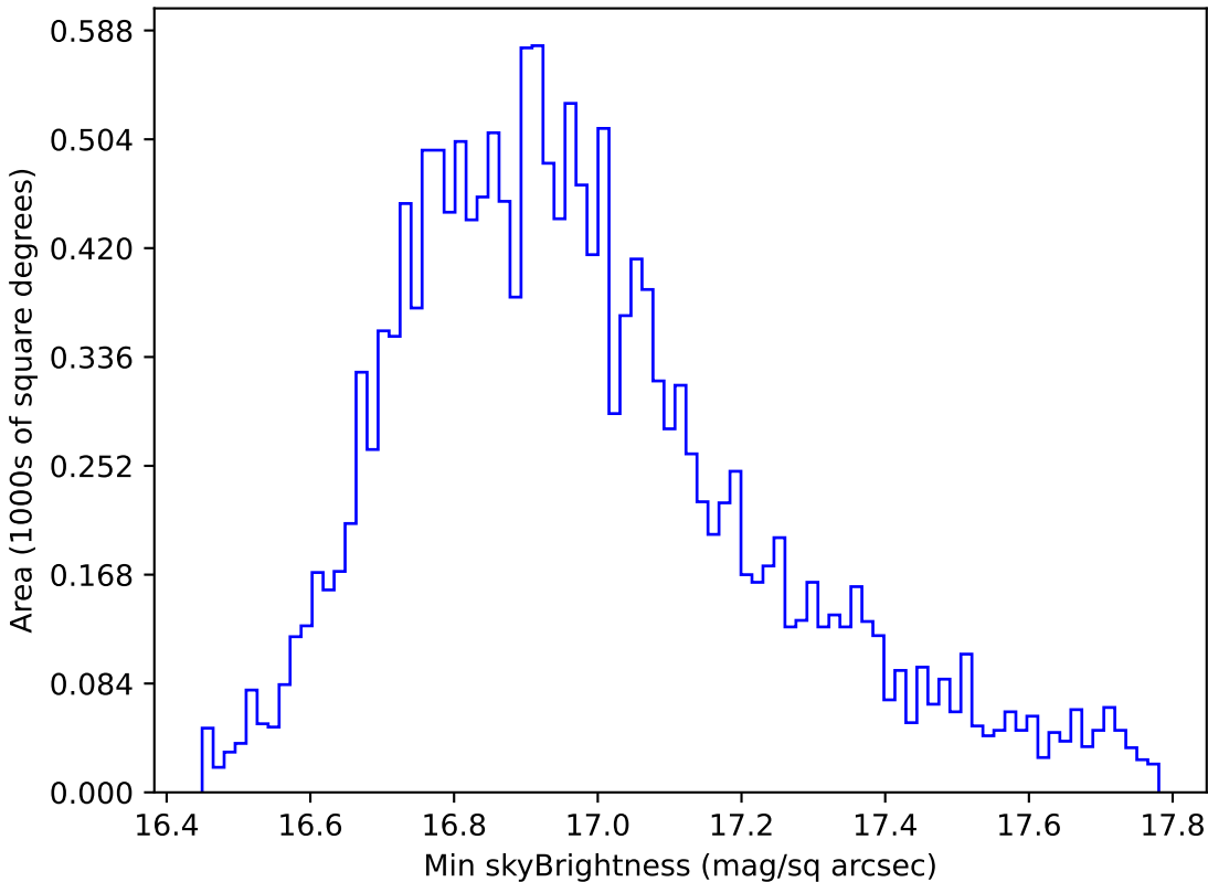
noroll_v3.4_10yrs WFD all bands: Min skyBrightness
