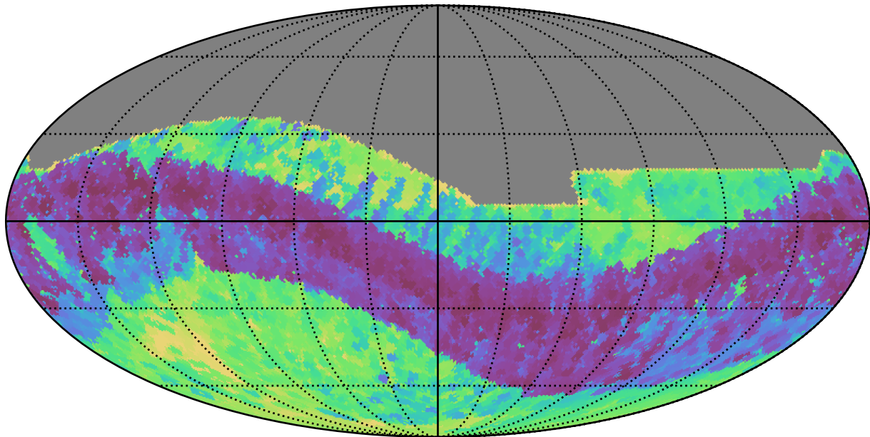
noroll_v3.4_10yrs All sky z band: Min skyBrightness
