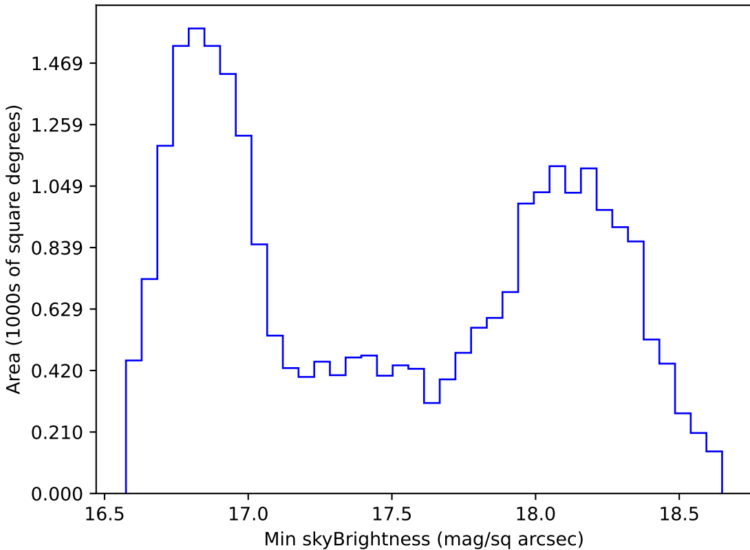
noroll_v3.4_10yrs All sky z band: Min skyBrightness
