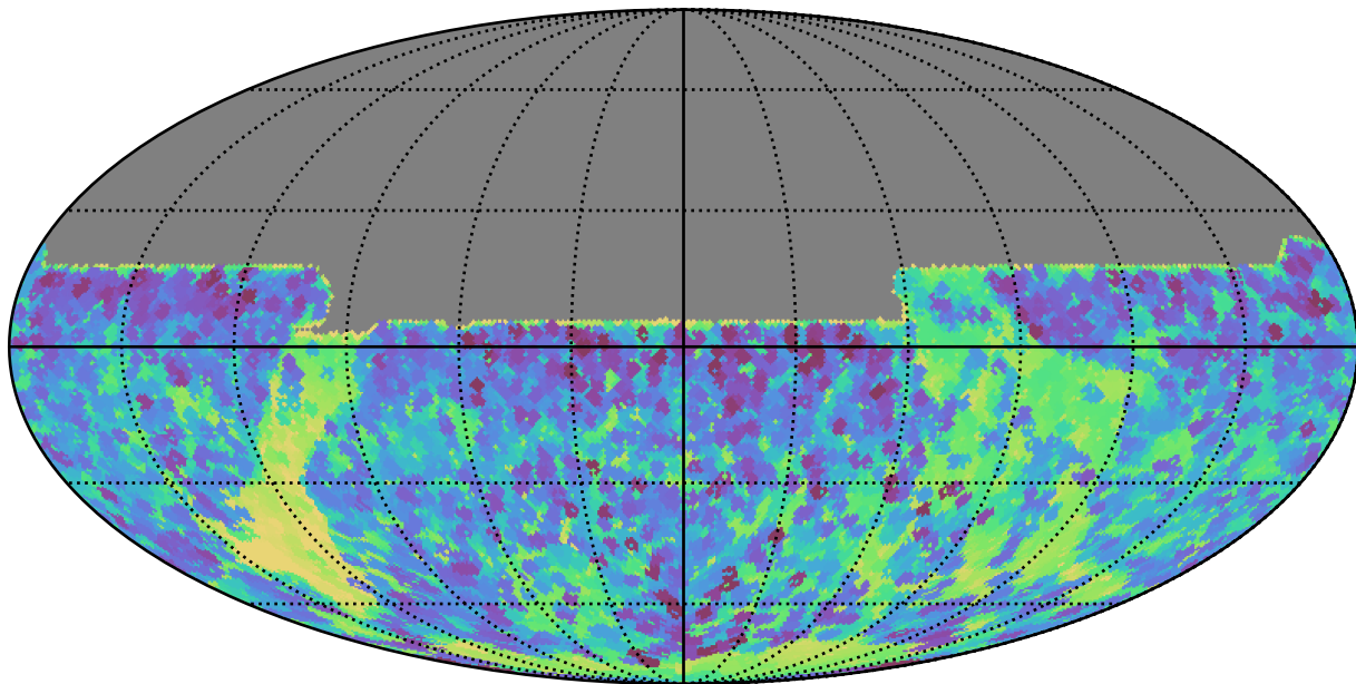
noroll_v3.4_10yrs All sky y band: Min skyBrightness
