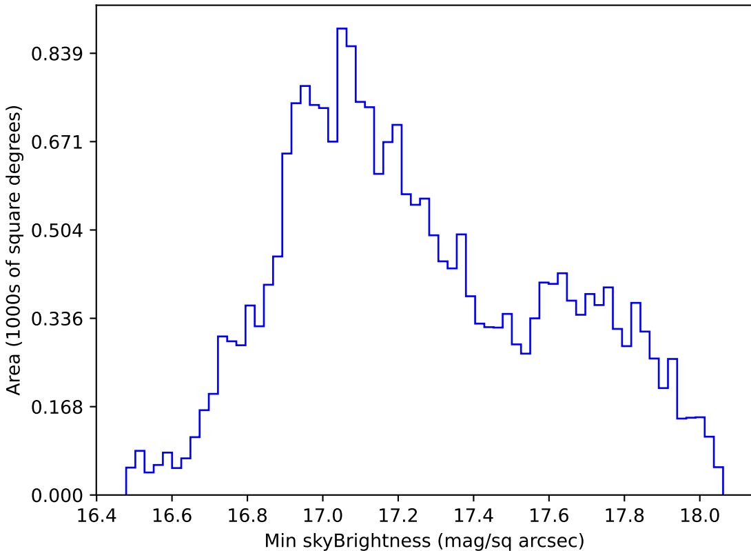
noroll_v3.4_10yrs All sky y band: Min skyBrightness
