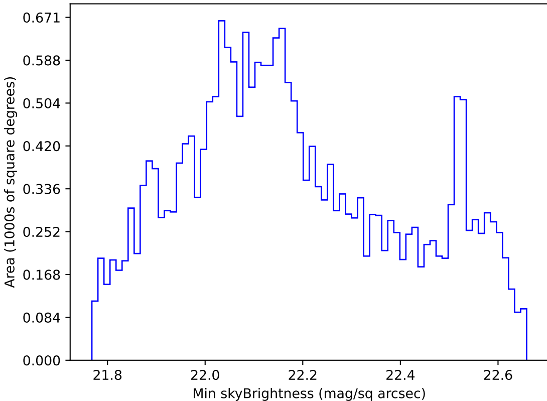
noroll_v3.4_10yrs All sky u band: Min skyBrightness
