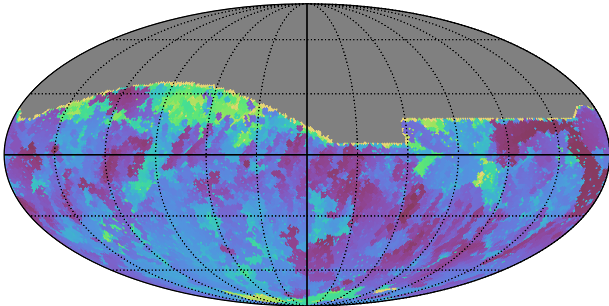
noroll_v3.4_10yrs All sky r band: Min skyBrightness
