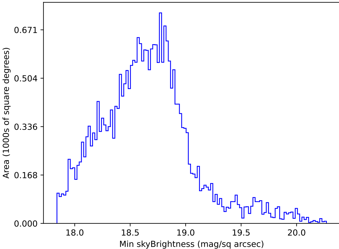
noroll_v3.4_10yrs All sky r band: Min skyBrightness
