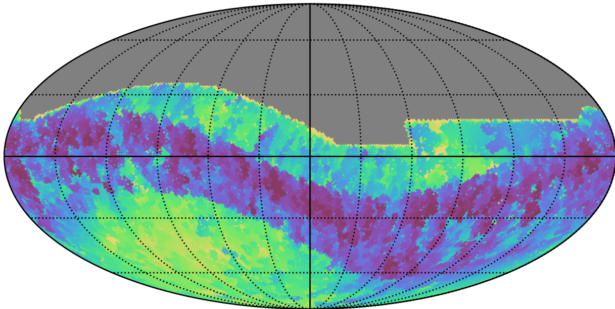
noroll_v3.4_10yrs All sky i band: Min skyBrightness
