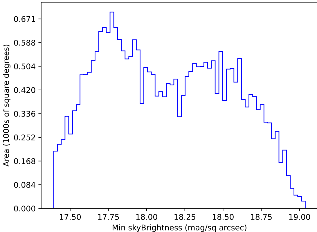
noroll_v3.4_10yrs All sky i band: Min skyBrightness
