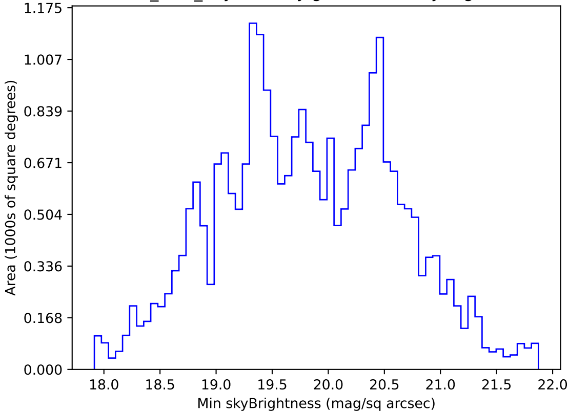
noroll_v3.4_10yrs All sky g band: Min skyBrightness
