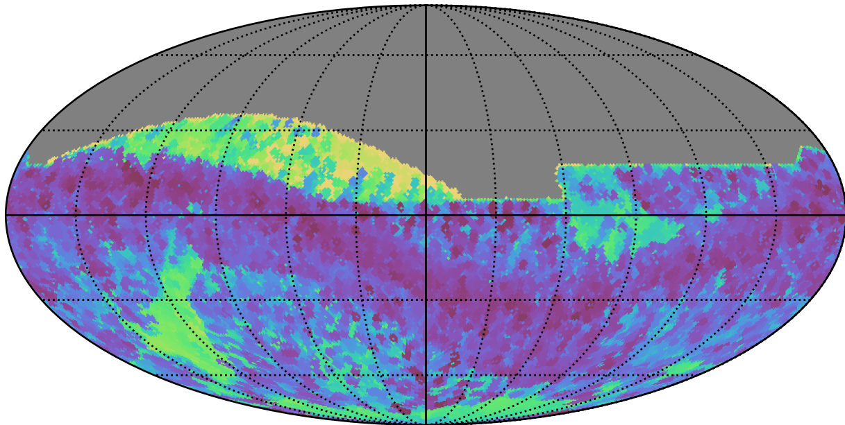
noroll_v3.4_10yrs All sky all bands: Min skyBrightness
